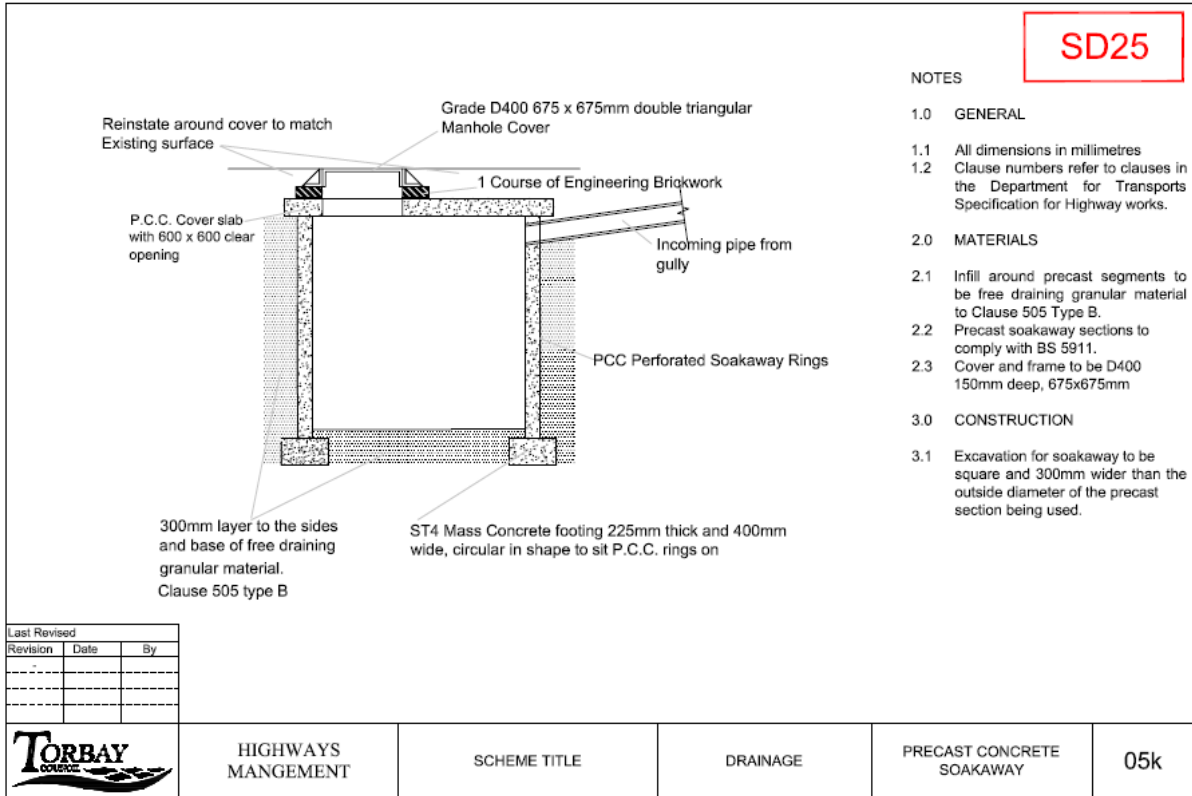
TYPICAL SOAKAWAY DETAILS
