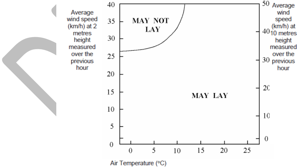
FIGURE 7/2: Wind Speed and Air Temperature Laying Restraints for Dense Concrete Asphalt Surface Course or Binder Course
