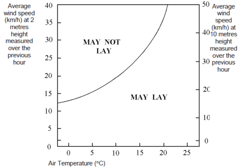
FIGURE 7/2: Wind Speed and Air Temperature Laying Restraints for Dense Concrete Asphalt Surface Course or Binder Course
